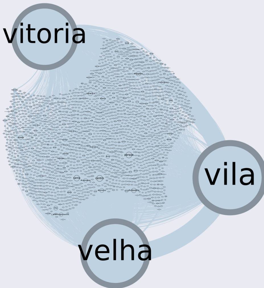
Cluster 02 - word_graph
