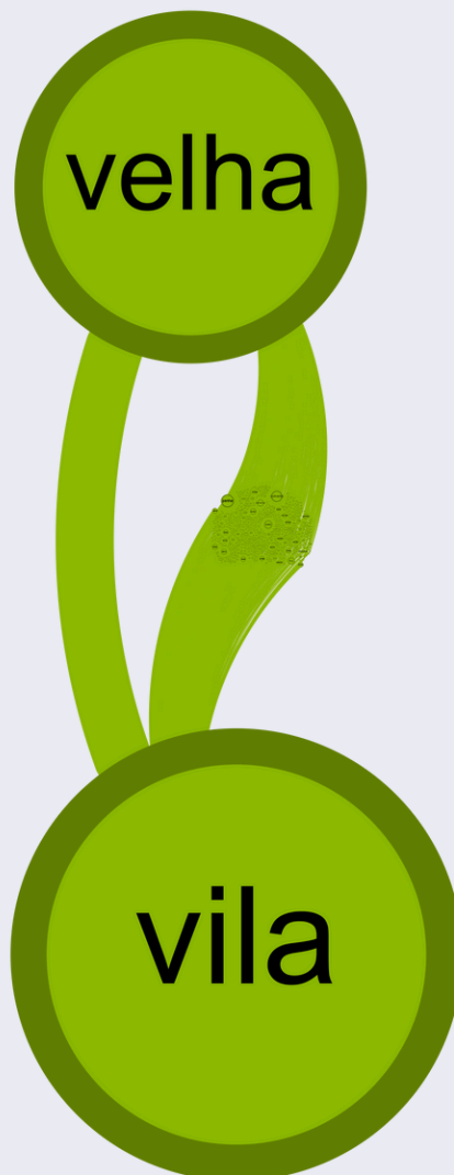
Cluster 02- word_graph
