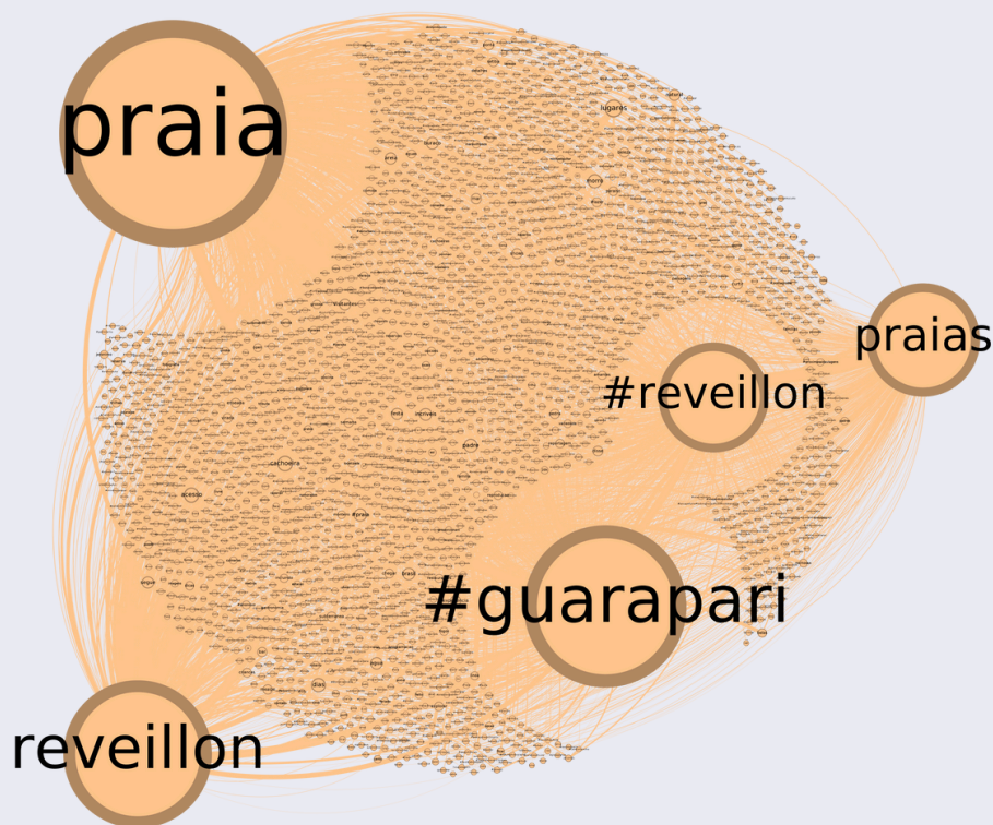
Cluster 01 - word_graph
